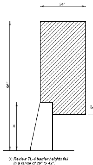
Figure 4.2.5-8 Sign Support Bracket Shy Distance
