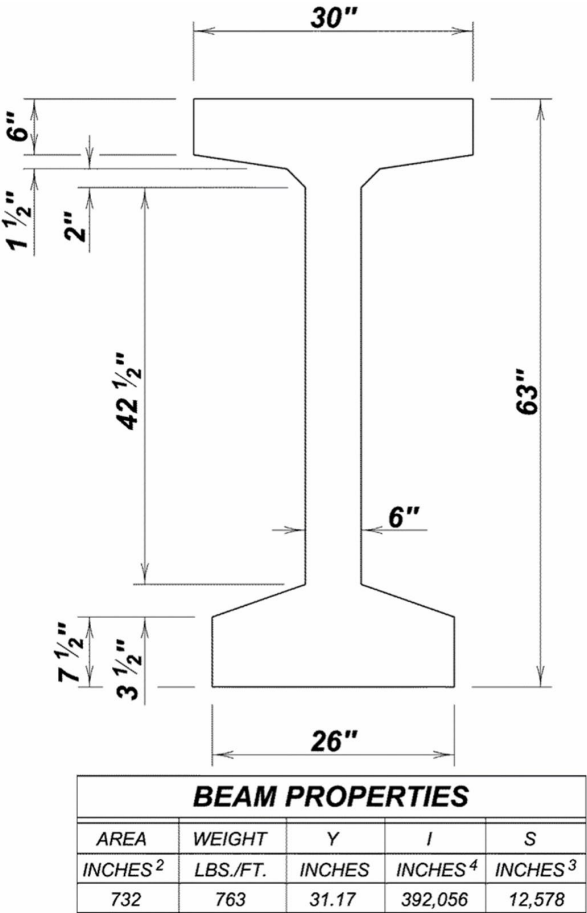
Figure 4.2.5-16 63M Prestressed Girder Properties
