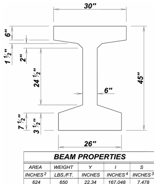
Figure 4.2.5-14 45M Prestressed Girder Properties
