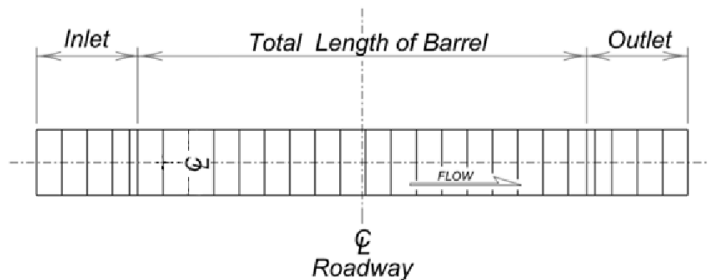
Figure 4.1.2-3 Precast Box Culvert Length Layout
