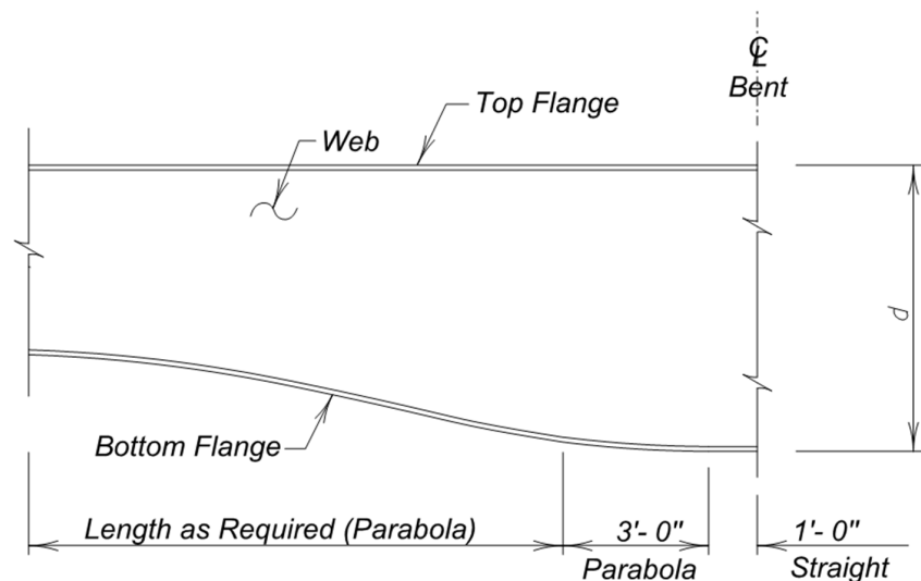
Figure 4.2.5-19 Parabolic Haunch Steel Girder
