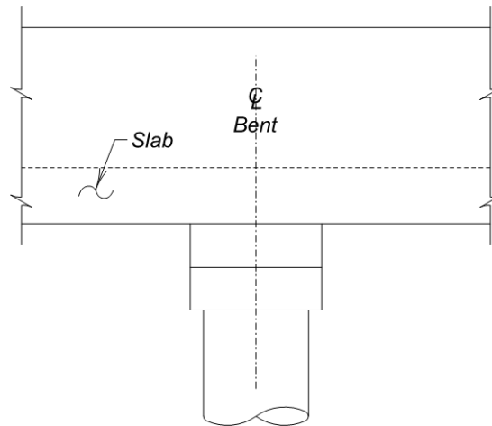
Figure 4.2.5-11 Flat Slab Continuous Concrete Bridge
