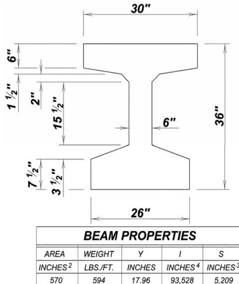
Figure 4.2.5-13 36M Prestressed Girder Properties
