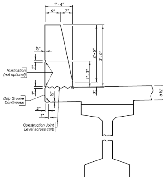
Figure 4.2.5-3 Single Slope Concrete Bridge Rail
