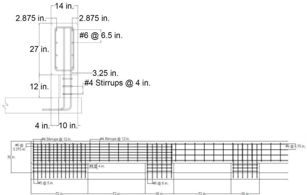
Figure 4.2.5-5 Open Concrete Bridge Rail
