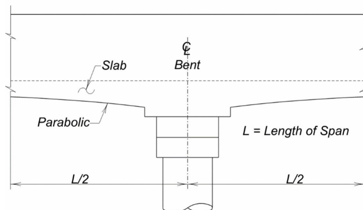
Figure 4.2.5-10 Parabolic Haunch Slab Continuous Concrete Bridge
