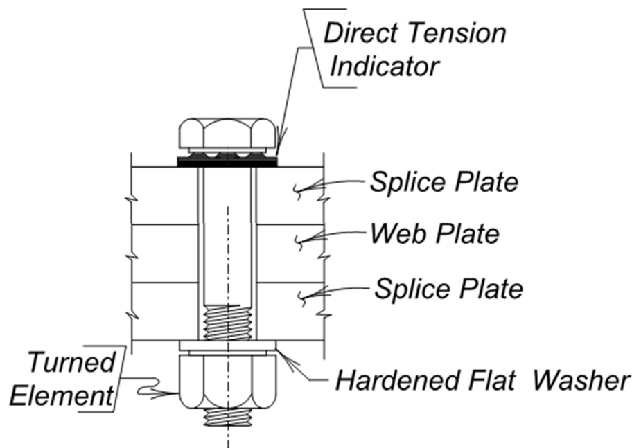
Figure 4.2.5-21 Bolt and Direct Tension Indicator Details for Bolted Field Splice
