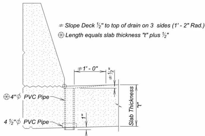
Figure 4.2.5-6 Deck Drain Detail Continuous Concrete Bridge
