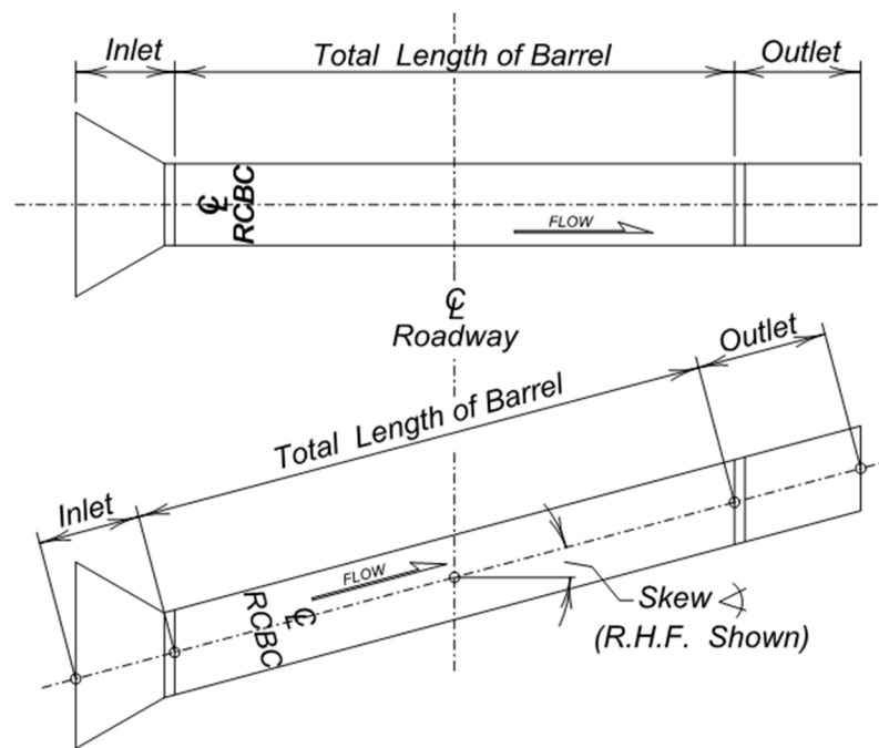
Figure 4.1.2-2 Cast in Place Box Culvert Length Layout
