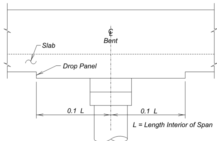
Figure 4.2.5-9 Drop Panel Haunch Slab Continuous Concrete Bridge
