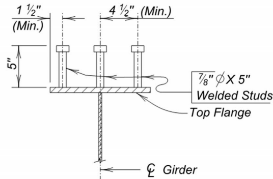
Figure 4.2.5-22 Shear Stud Connection Detail
