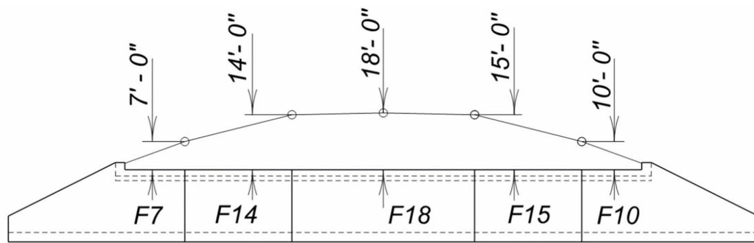
Figure 4.1.2-5 Box Culvert Fill Height Designation
