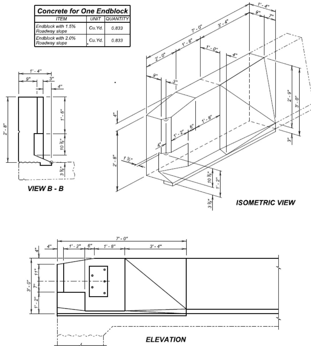
Figure 4.2.5-4 Single Slope Concrete Bridge Rail End Block
