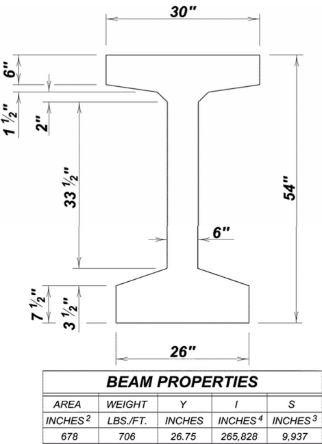
Figure 4.2.5-15 54M Prestressed Girder Properties
