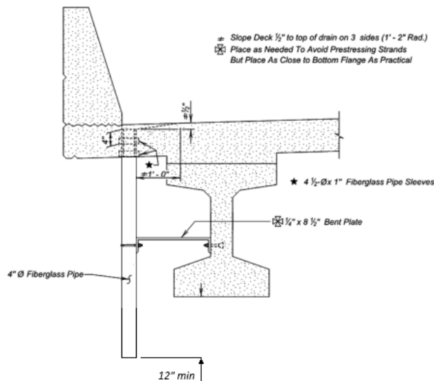
Figure 4.2.5-7 Deck Drain Details Girder Bridge
