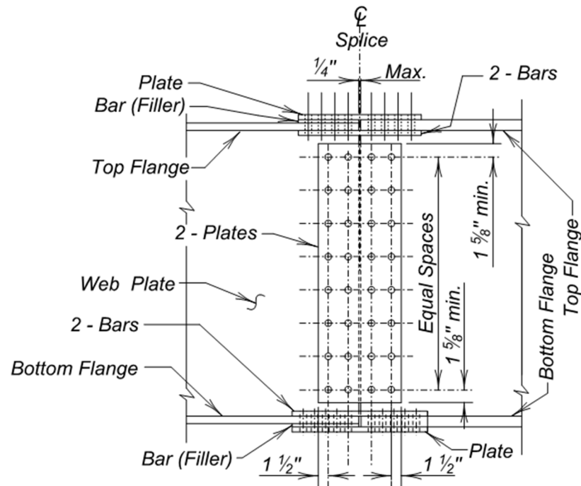
Figure 4.2.5-20 Bolted Field Splice Detail
