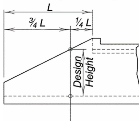
Figure 4.2.4-4 Wingwall Design Height
