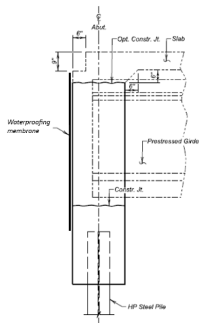
Figure 4.2.6-1 Integral Abutment Prestressed Girder Bridge Sept 2025
