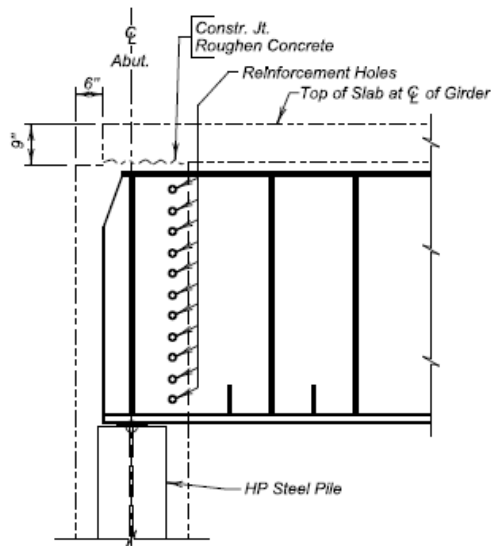
Figure 4.2.6-2 Integral Abutment Steel Girder Bridge
