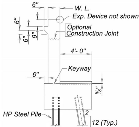
Figure 4.2.6-4 Sill Type Abutment Girder Bridge
