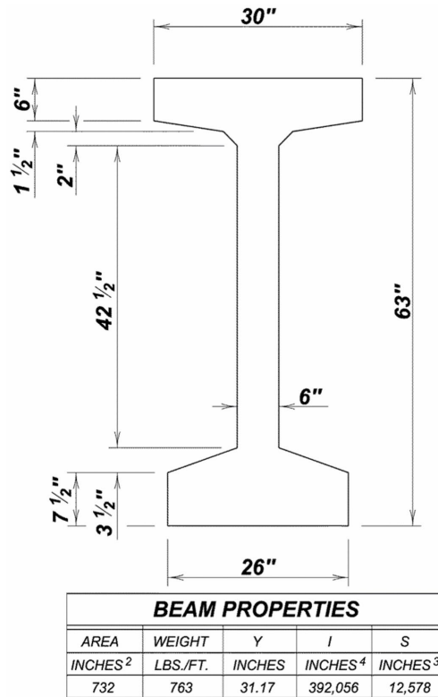
Figure 4.2.5 - 16 63M Prestressed Girder Properties
