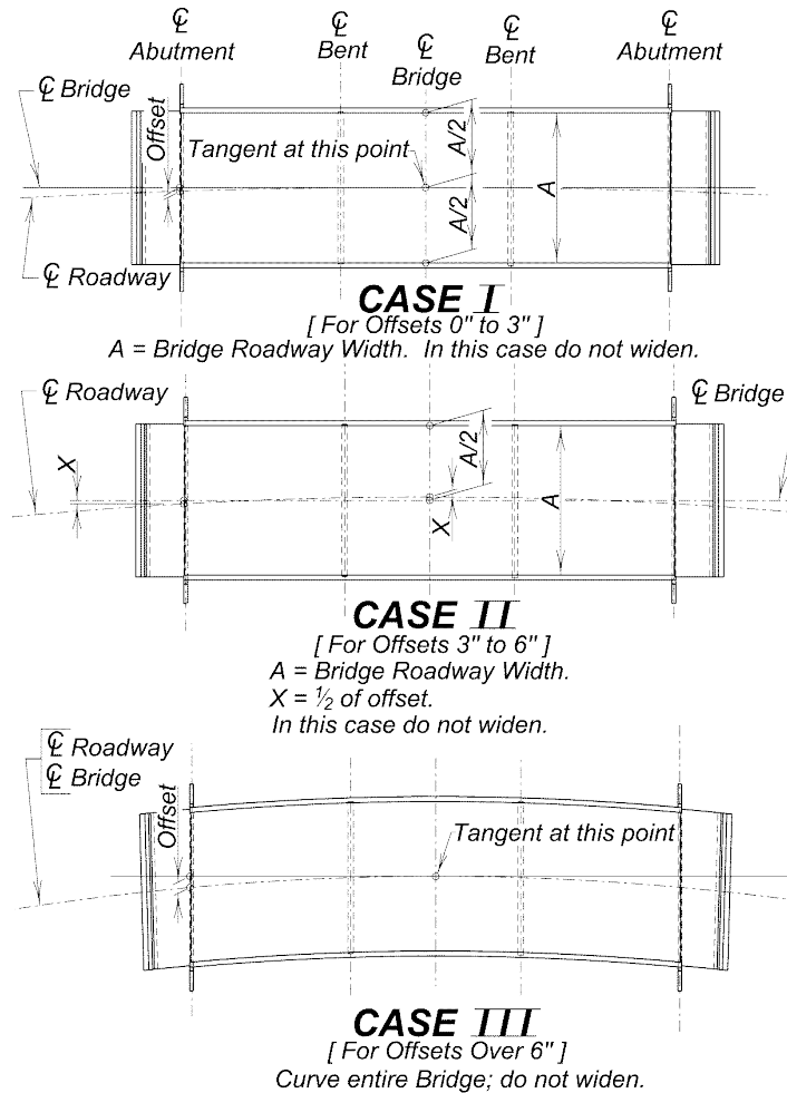
Figure 4.1.1 - 1 Bridge Alignment for Horizontal Curve
