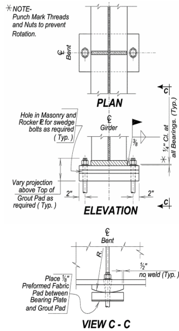
Figure 4.2.5 - 1 Steel Girder Fixed Rocker Bearing
