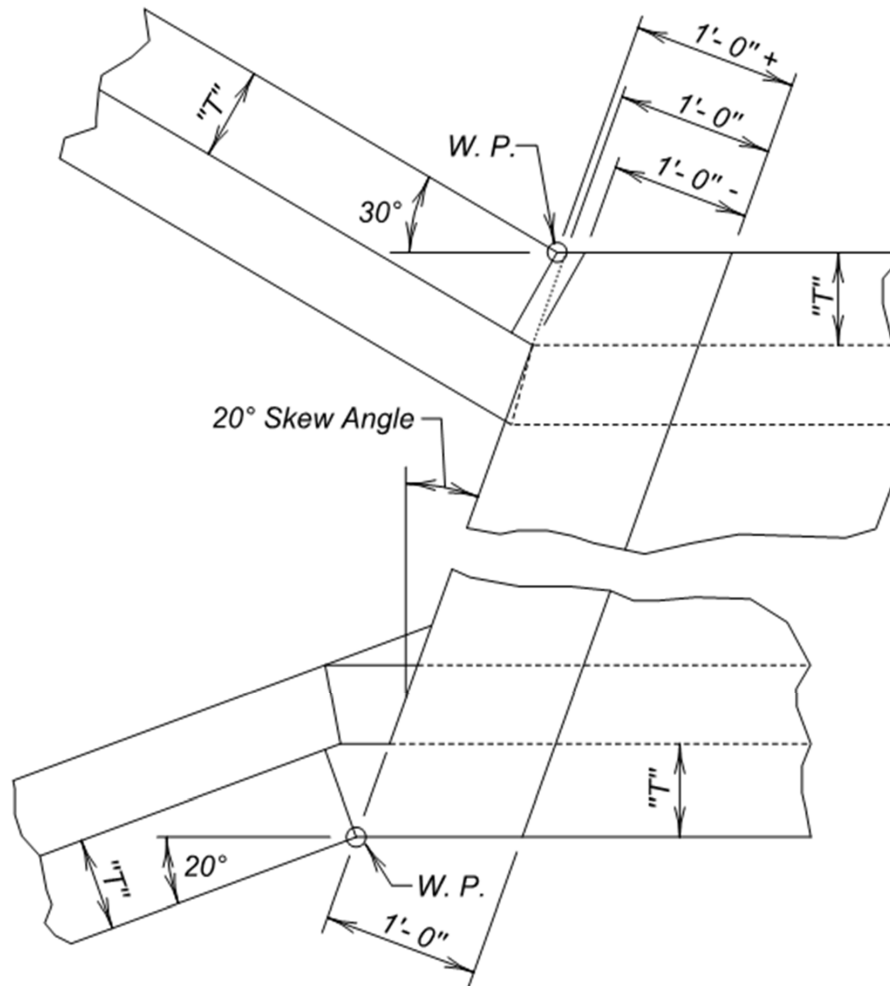
Figure 4.1.2 - 8 Cast in Place Box Culvert Working Points
