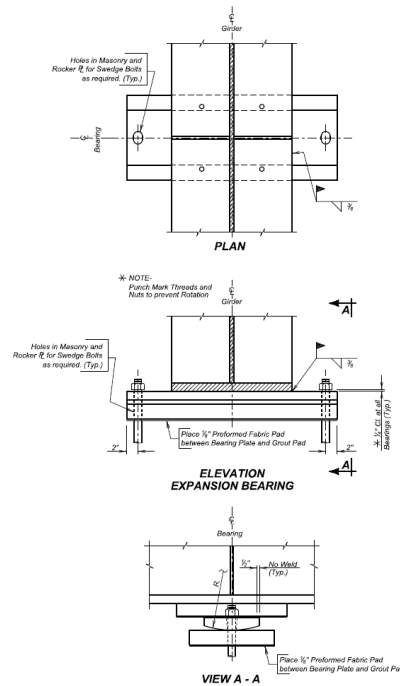
Figure 4.2.5 - 2 Steel Girder Expansion Rocker Bearing
