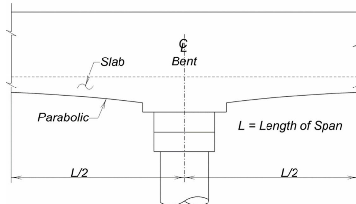
Figure 4.2.5 - 11 Parabolic Haunch Continuous Concrete Bridge
