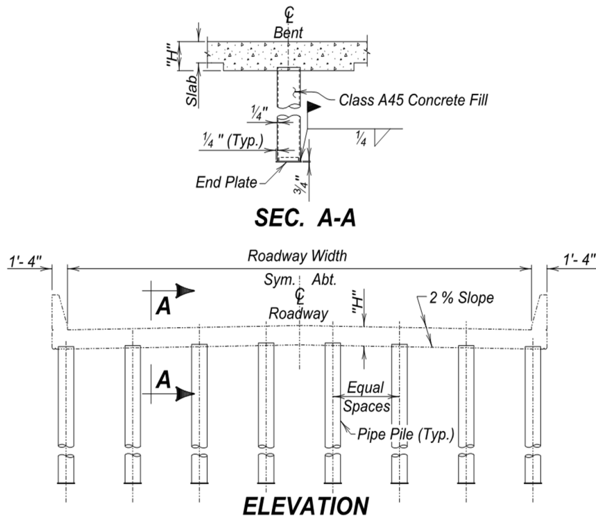
Figure 4.1.1 - 8 Steel Pipe Bent Continuous Concrete Bridge
