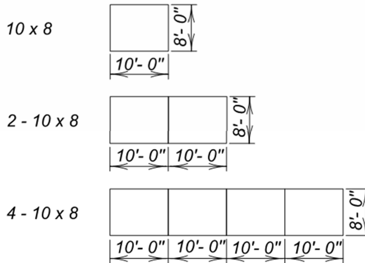
Figure 4.1.2 - 1 Box Culvert Cell Layout
