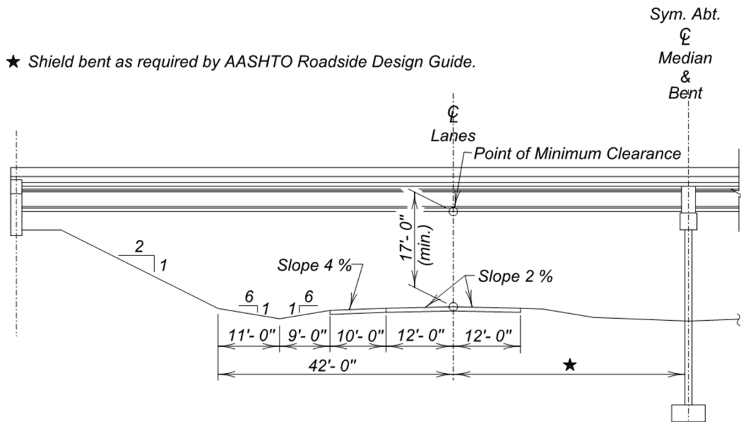
Figure 4.1.2 - 11 Structure Over Rural Interstate Highway
