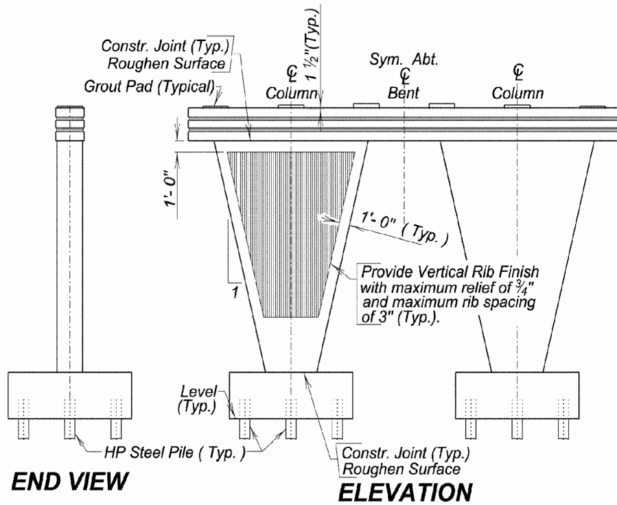
Figure 4.1.1 - 7 Alternate Two Column Bent Girder Bridge
