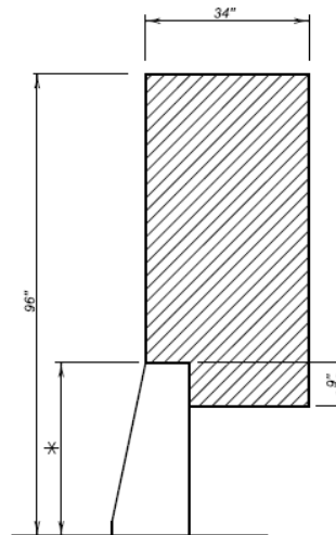
Figure 4.2.5 - 9 Sign Support Bracket Shy Distance
