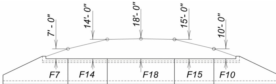
Figure 4.1.2 - 5 Box Culvert Fill Height Designation
