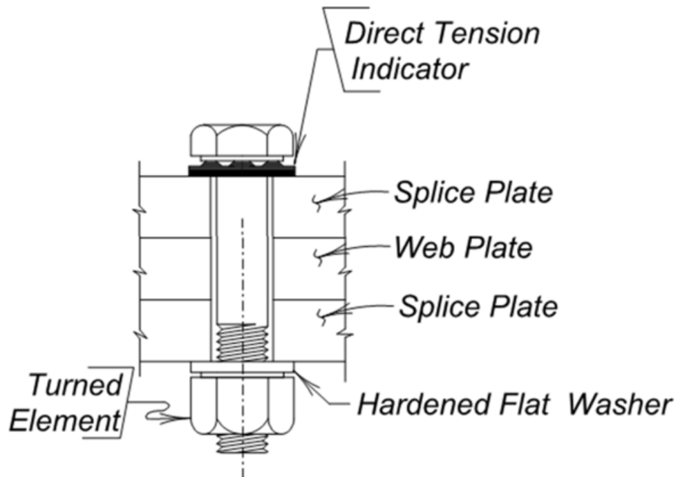
Figure 4.2.5 - 21 Direct Tension Indicator Details
