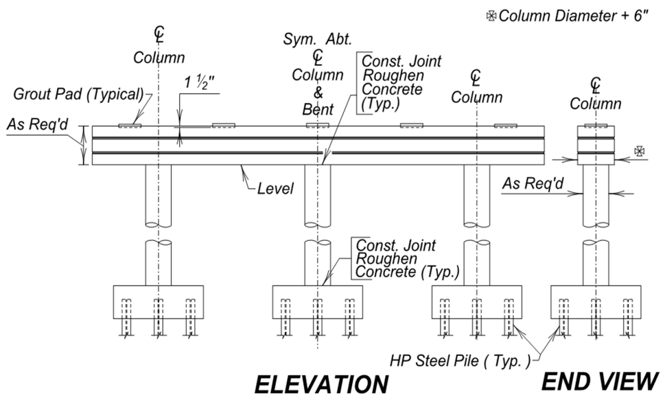
Figure 4.1.1 - 4 Three Column Bent Girder Bridge
