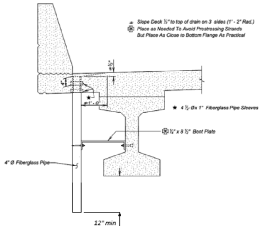
Figure 4.2.5 - 7 Deck Drain Details, Girder Bridge
