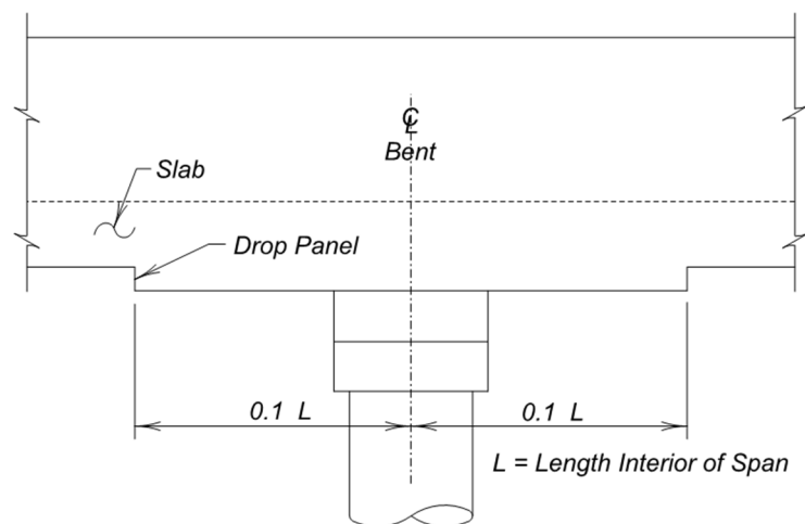
Figure 4.2.5 - 10 Drop Panel Haunch Continuous Concrete Bridge
