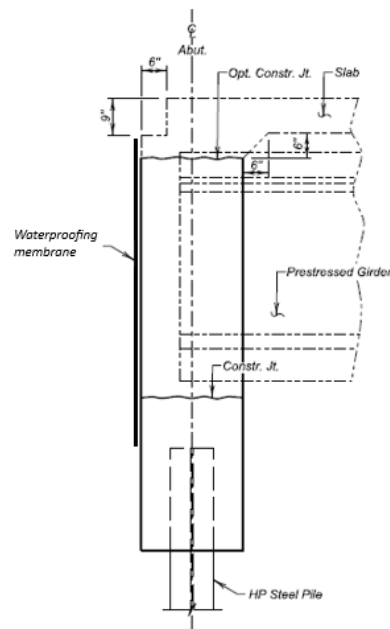
Figure 4.2.6 - 1 Integral Abutment Prestressed Girder Bridge
