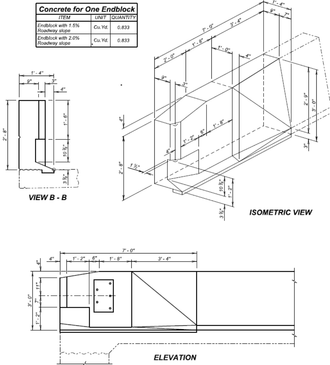
Figure 4.2.5 - 4 Single Slope Concrete Bridge Rail End Block
