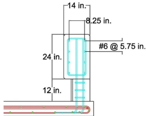
Figure 4.2.5 - 5 Open Concrete Bridge Rail
