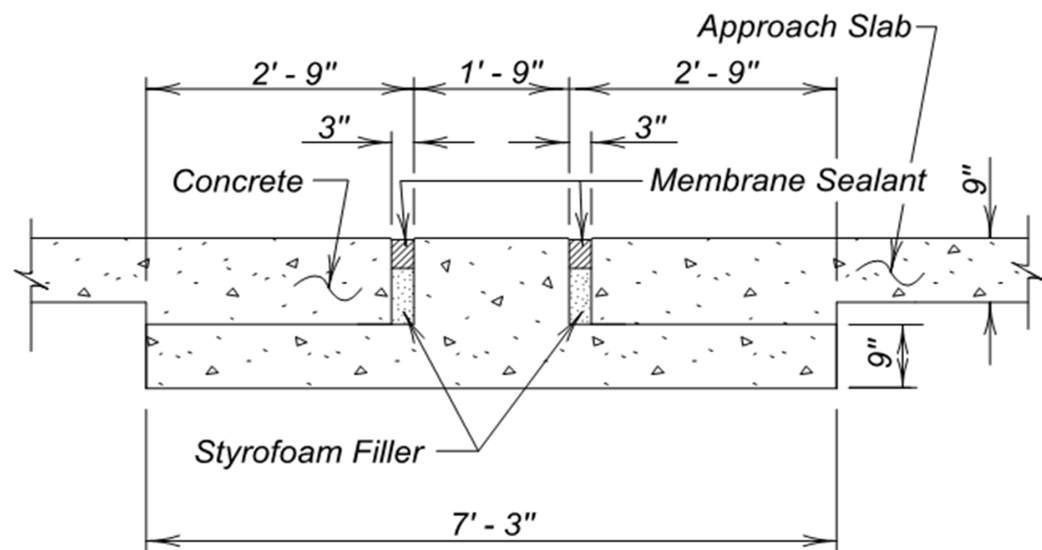
Figure 4.1.1 - 10 Hat Type Sleeper Slab (For Use with Concrete Approach Pavement and Integral Abutment)
