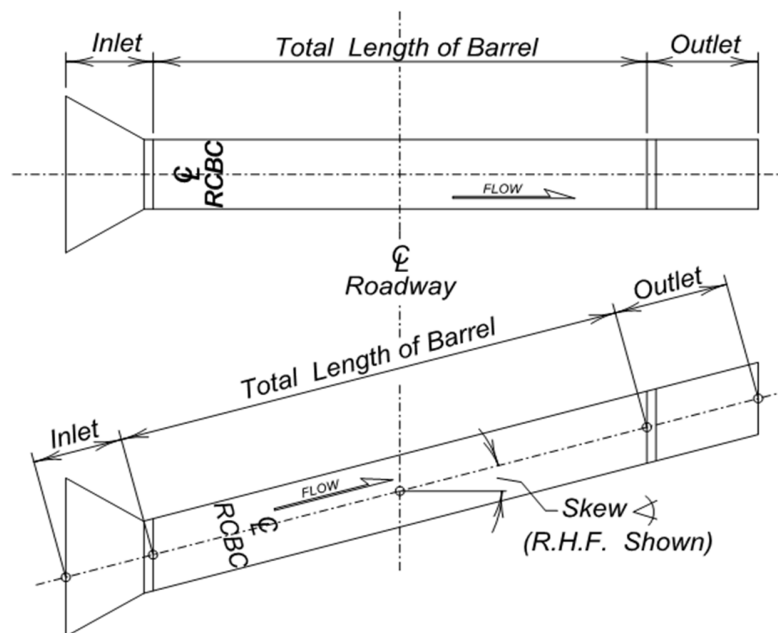
Figure 4.1.2 - 2 Cast in Place Box Culvert Length Layout
