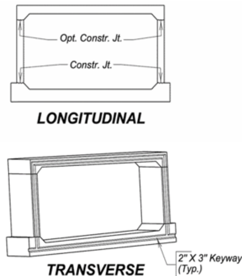
Figure 4.2.4 - 5 Box Culvert Construction Joints
