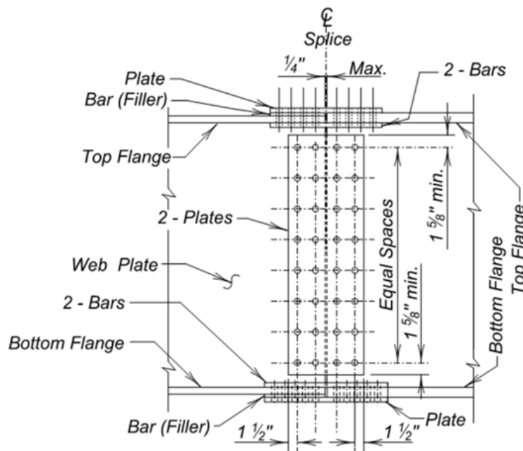
Figure 4.2.5 - 20 Bolted Field Splice Detail
