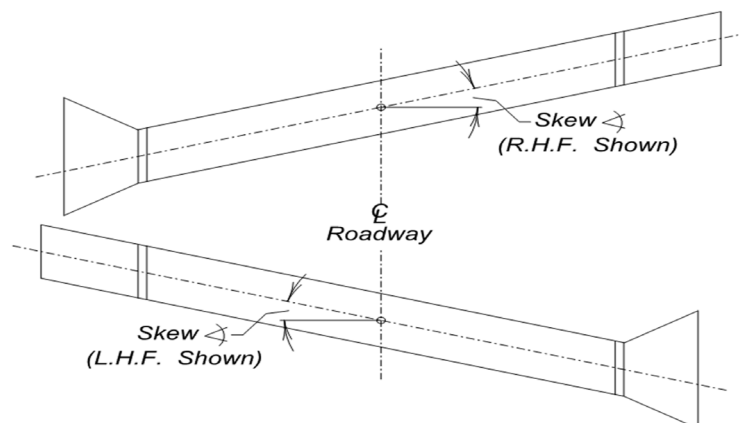
Figure 4.1.2 - 6 RHF and LHF Box Culvert Skew
