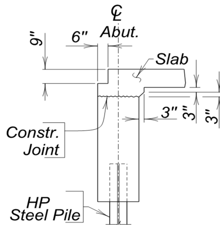
Figure 4.2.6 - 3 Integral Abutment Continuous Concrete Bridge
