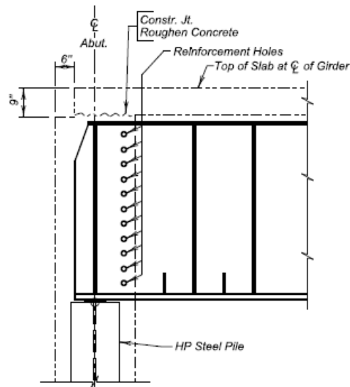
Figure 4.2.6 - 2 Integral Abutment Steel Girder Bridge
