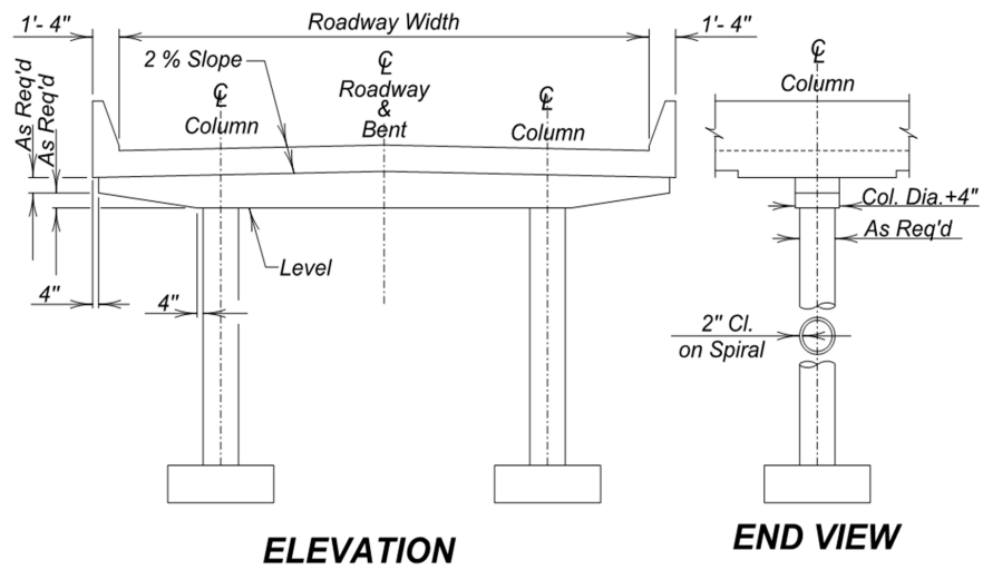
Figure 4.1.1 - 3 Two Column Bent Continuous Concrete Bridge
