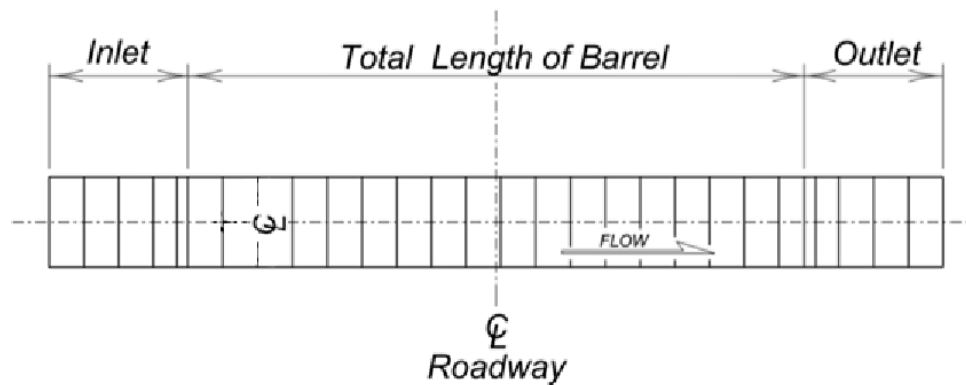
Figure 4.1.2 - 3 Precast Box Culvert Length Layout
