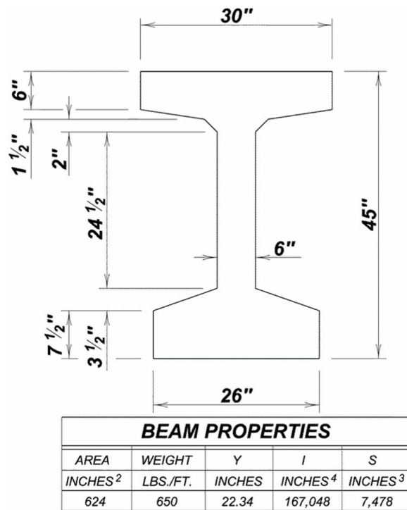
Figure 4.2.5 - 14 45M Prestressed Girder Properties
