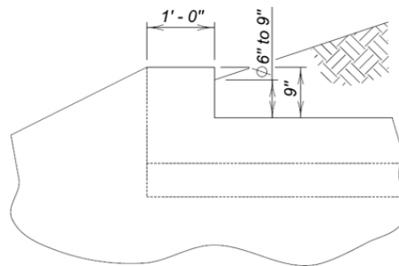
Figure 4.1.2 - 4 Inslope Parapet Intersection (Cast in Place)
