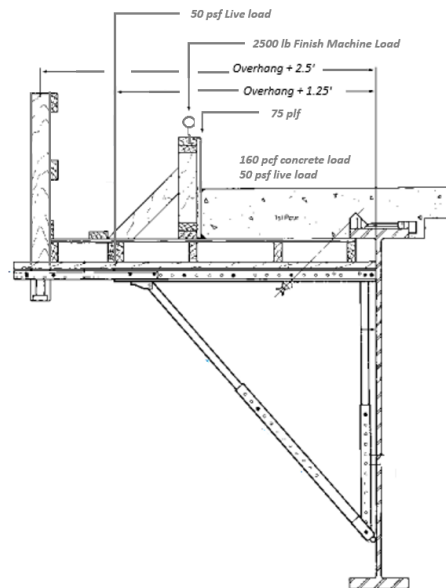
Figure 4.2.5 - 23 False Work Overhang Bracket
