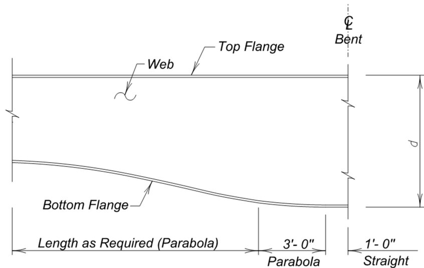
Figure 4.2.5 - 19 Parabolic Haunch Steel Girder
