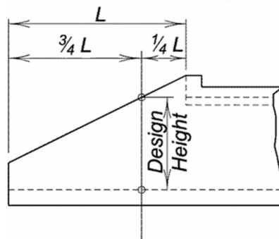
Figure 4.2.4 - 4 Wingwall Design Height
