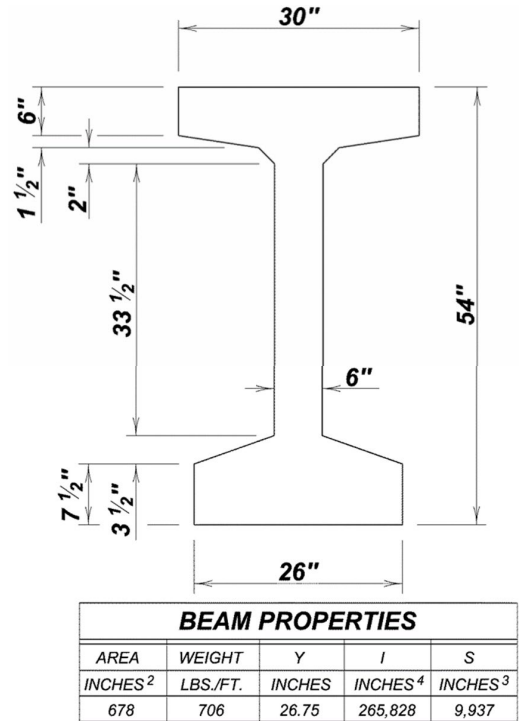
Figure 4.2.5 - 15 54M Prestressed Girder Properties
