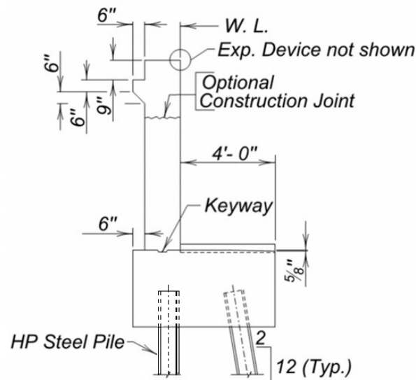
Figure 4.2.6 - 4 Sill Type Abutment for Girder Bridges
