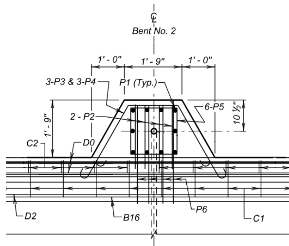
Figure 4.2.5 - 8 Pole Support on Bridge Rail
