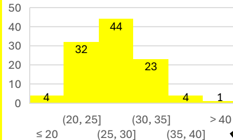
Car Speed Observed at Location 2 (mph)
