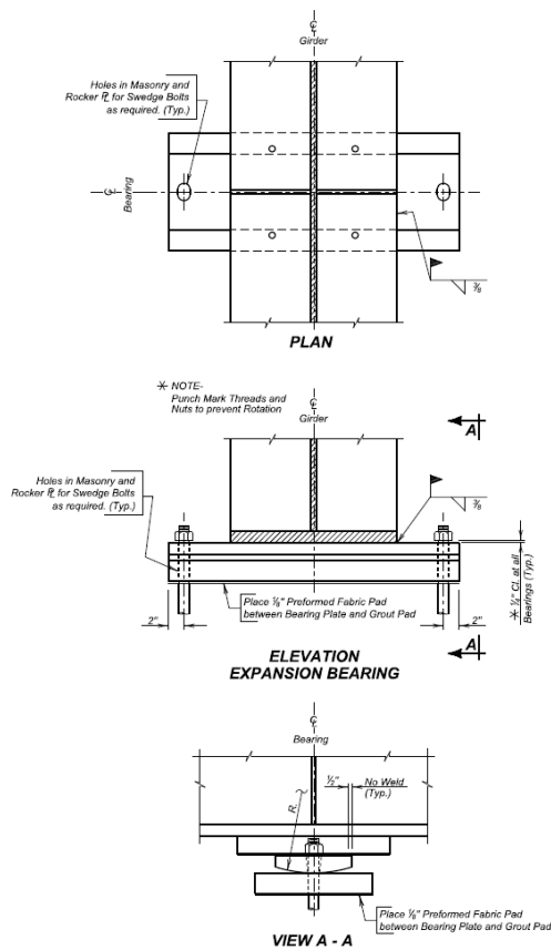
Figure 4.2.5-2 Steel Girder expansion Rocker Bearing Sept 2025
