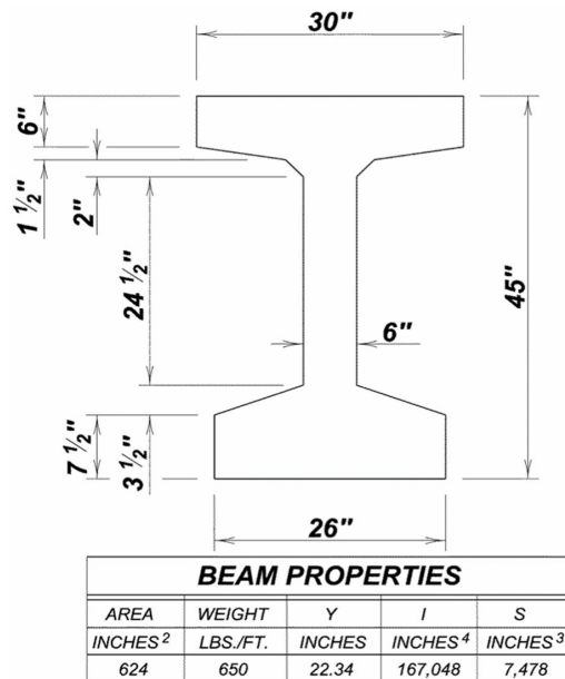
Figure 4.2.5-14 45M Prestressed Girder Properties
