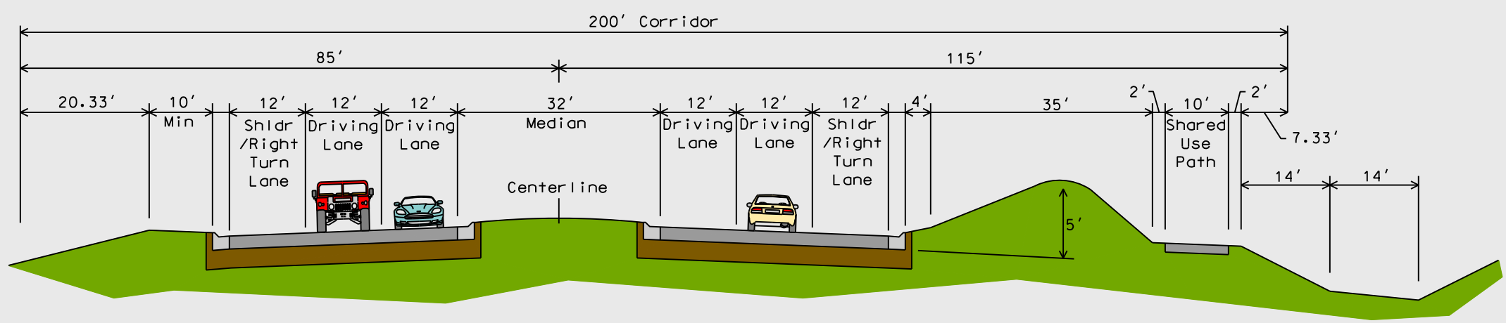
Section A Typical Section
